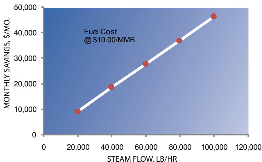
Typical performance of an EconoStak economizer.
